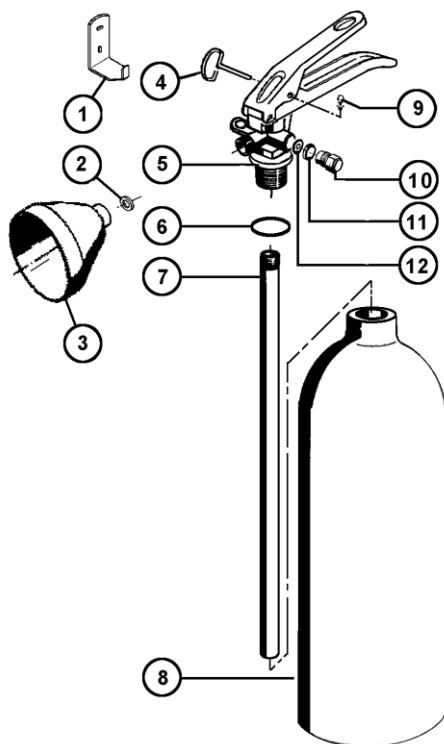
DESPIECE NC2
