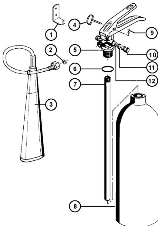
DESPIECE NC5
